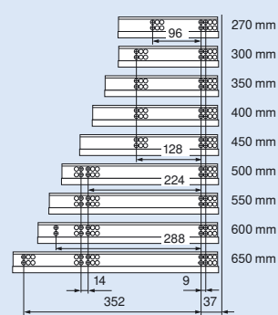
Hole pattern 550H
